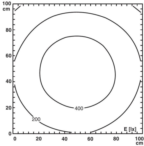
Figure 1 Illuminance distribution (Distance d = 1 m)
